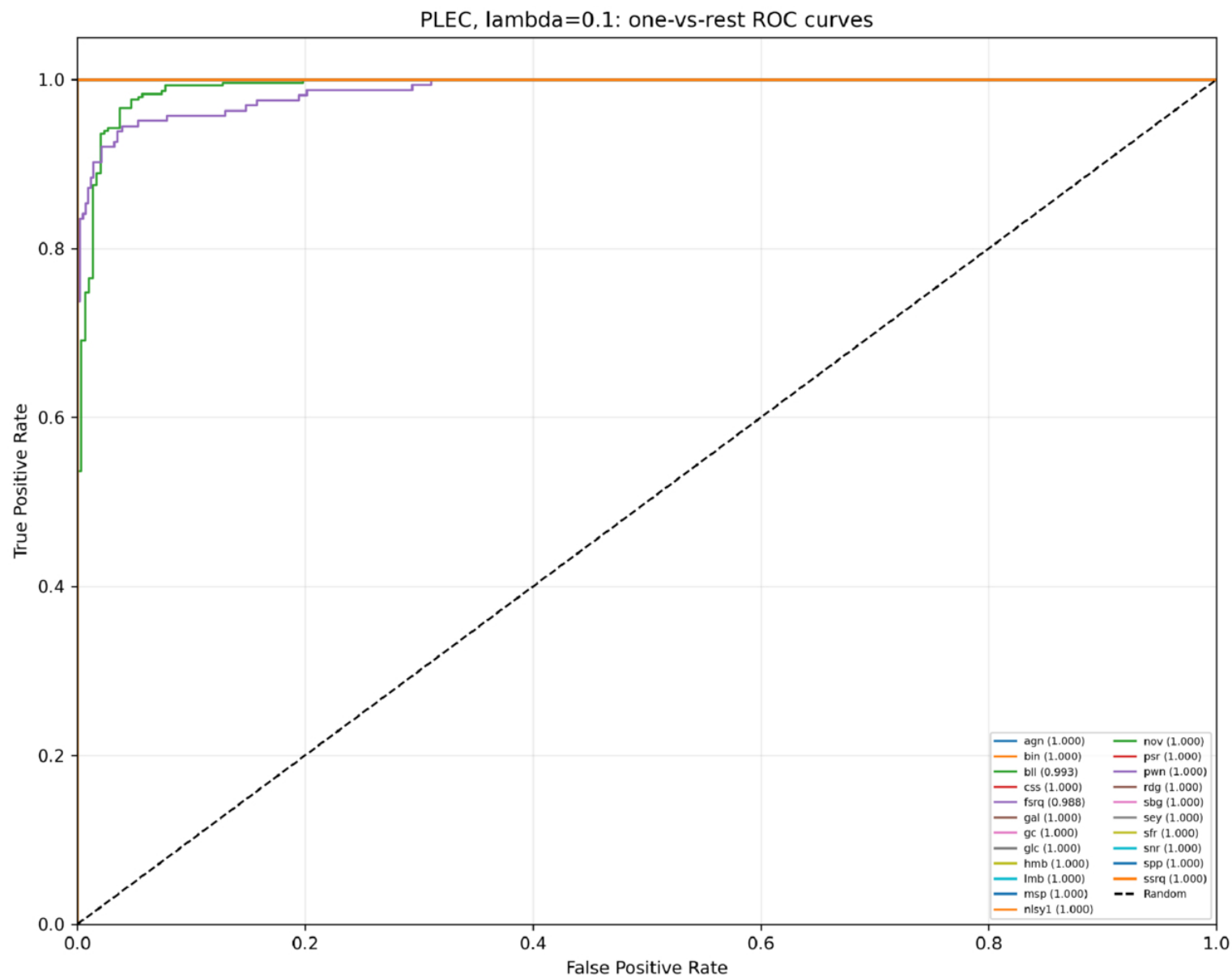
Figure 6. from Jingtian Zhu et al 2026 Astrophys. J. Suppl. 286 doi:10.3847/1538-4365/ae91e8 https://dx.doi.org/10.3847/1538-4365/ae91e8 © 2026. The Author(s). Published by the American Astronomical Society.
