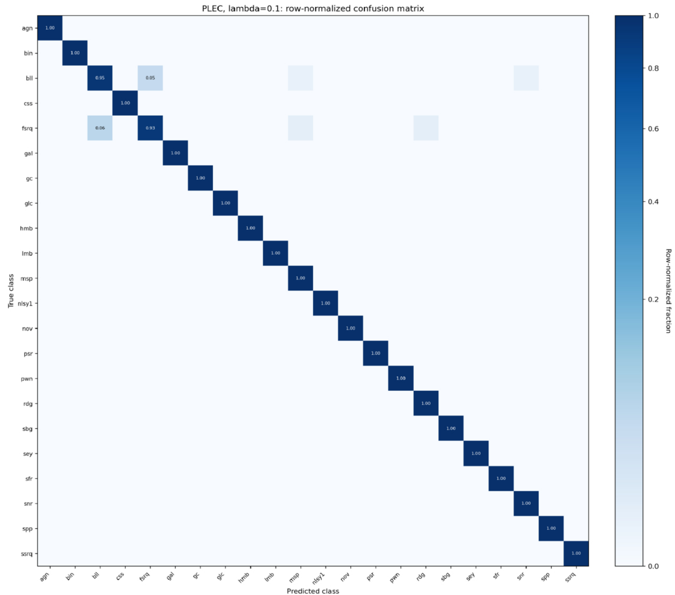
Figure 3. from Jingtian Zhu et al 2026 Astrophys. J. Suppl. 286 doi:10.3847/1538-4365/ae91e8 https://dx.doi.org/10.3847/1538-4365/ae91e8 © 2026. The Author(s). Published by the American Astronomical Society.
