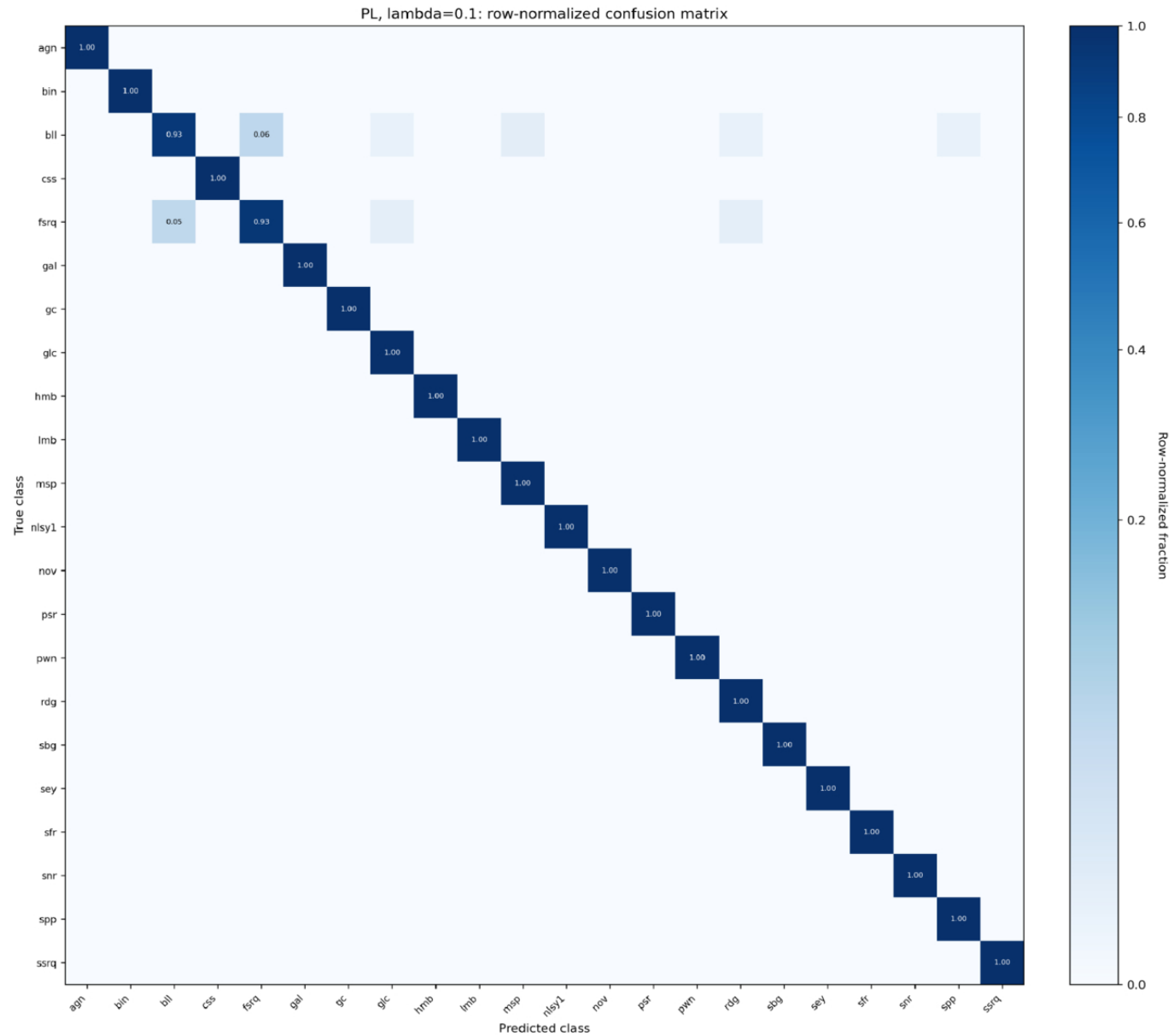
Figure 1. from Jingtian Zhu et al 2026 Astrophys. J. Suppl. 286 doi:10.3847/1538-4365/ae91e8 https://dx.doi.org/10.3847/1538-4365/ae91e8 © 2026. The Author(s). Published by the American Astronomical Society.
