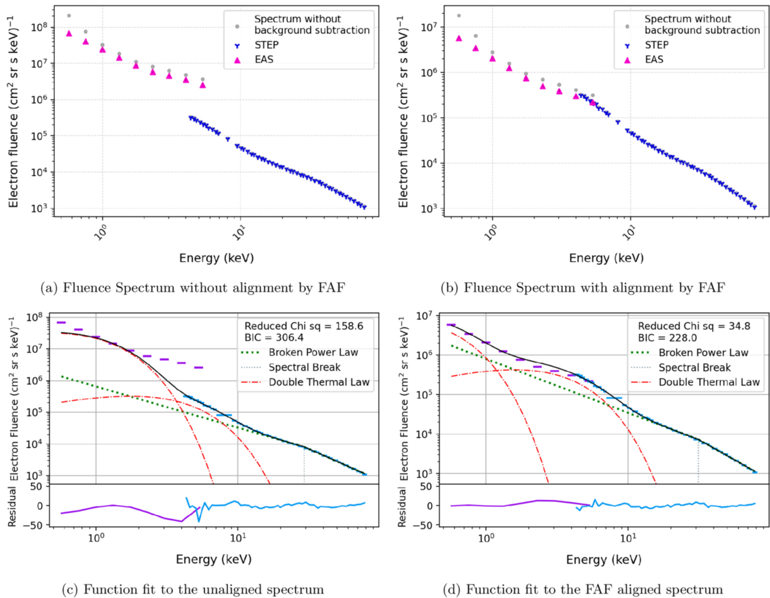
Figure 4. from Samuel Carter et al 2026 Astrophys. J. Suppl. 286 doi:10.3847/1538-4365/ae91e2 https://dx.doi.org/10.3847/1538-4365/ae91e2 © 2026. The Author(s). Published by the American Astronomical Society.
