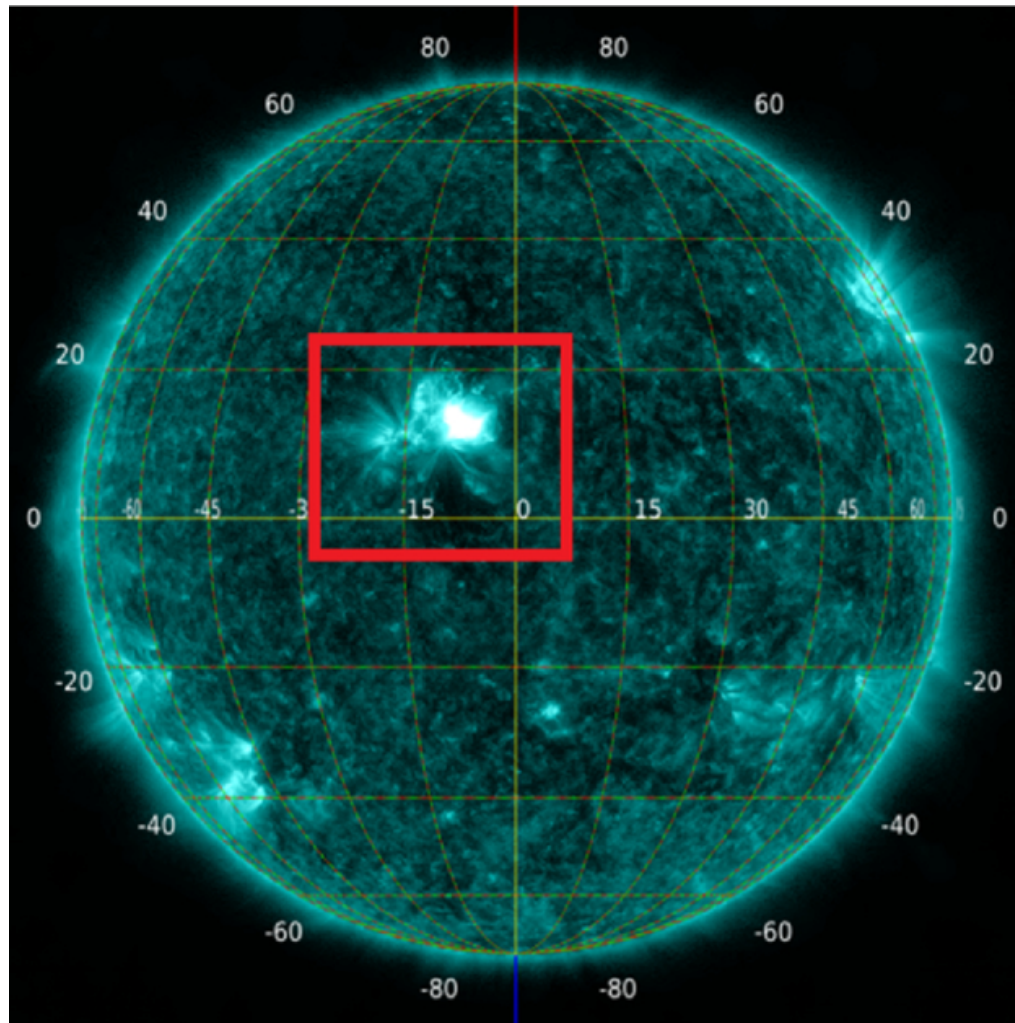
Figure 1. from Samuel Carter et al 2026 Astrophys. J. Suppl. 286 doi:10.3847/1538-4365/ae91e2 https://dx.doi.org/10.3847/1538-4365/ae91e2 © 2026. The Author(s). Published by the American Astronomical Society.
