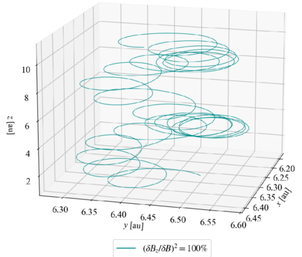
70 MeV proton trajectory segment
