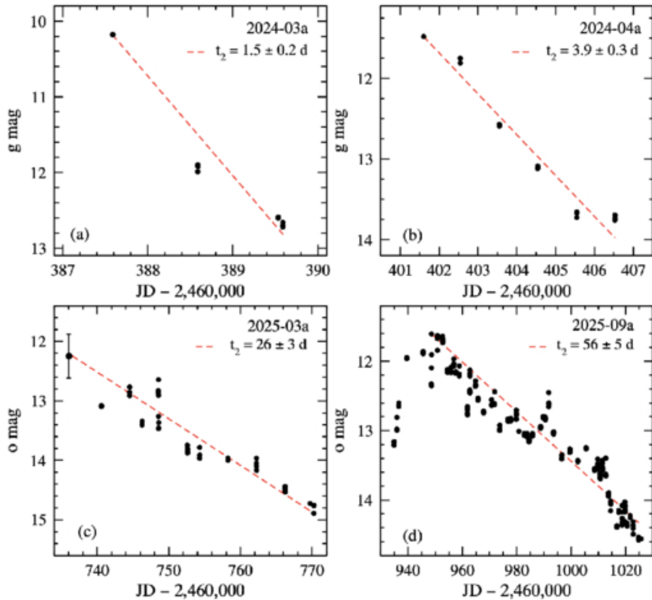
Figure 5. from Allen W. Shafter 2026 Astrophys. J. Suppl. 286 doi:10.3847/1538-4365/ae915a https://dx.doi.org/10.3847/1538-4365/ae915a © 2026. The Author(s). Published by the American Astronomical Society.
