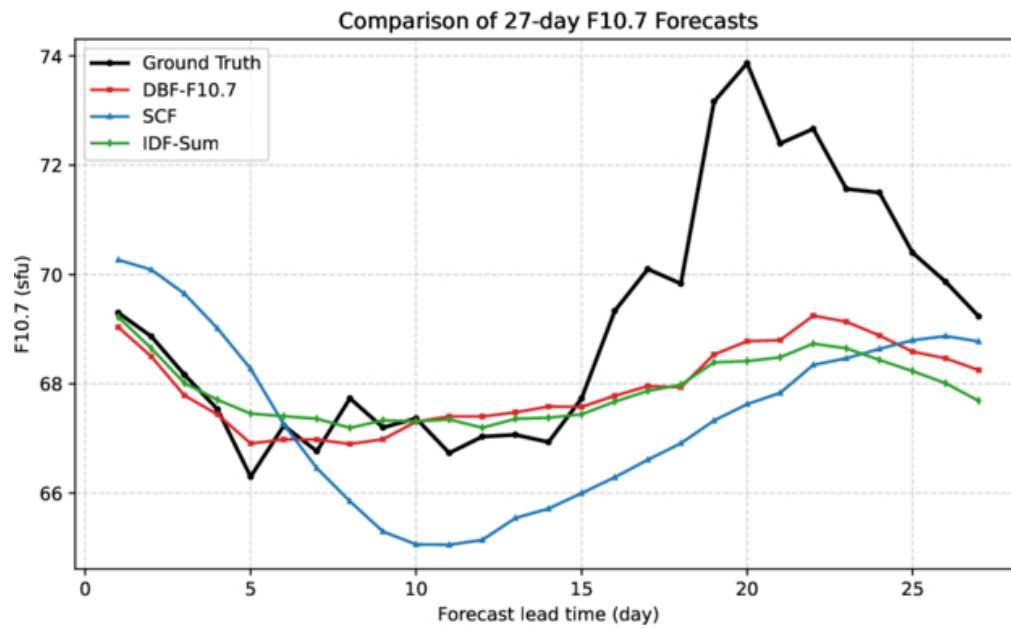
Figure 3. from Xiaolong Wang et al 2026 Astrophys. J. Suppl. 286 doi:10.3847/1538-4365/ae9096 https://dx.doi.org/10.3847/1538-4365/ae9096 © 2026. The Author(s). Published by the American Astronomical Society.
