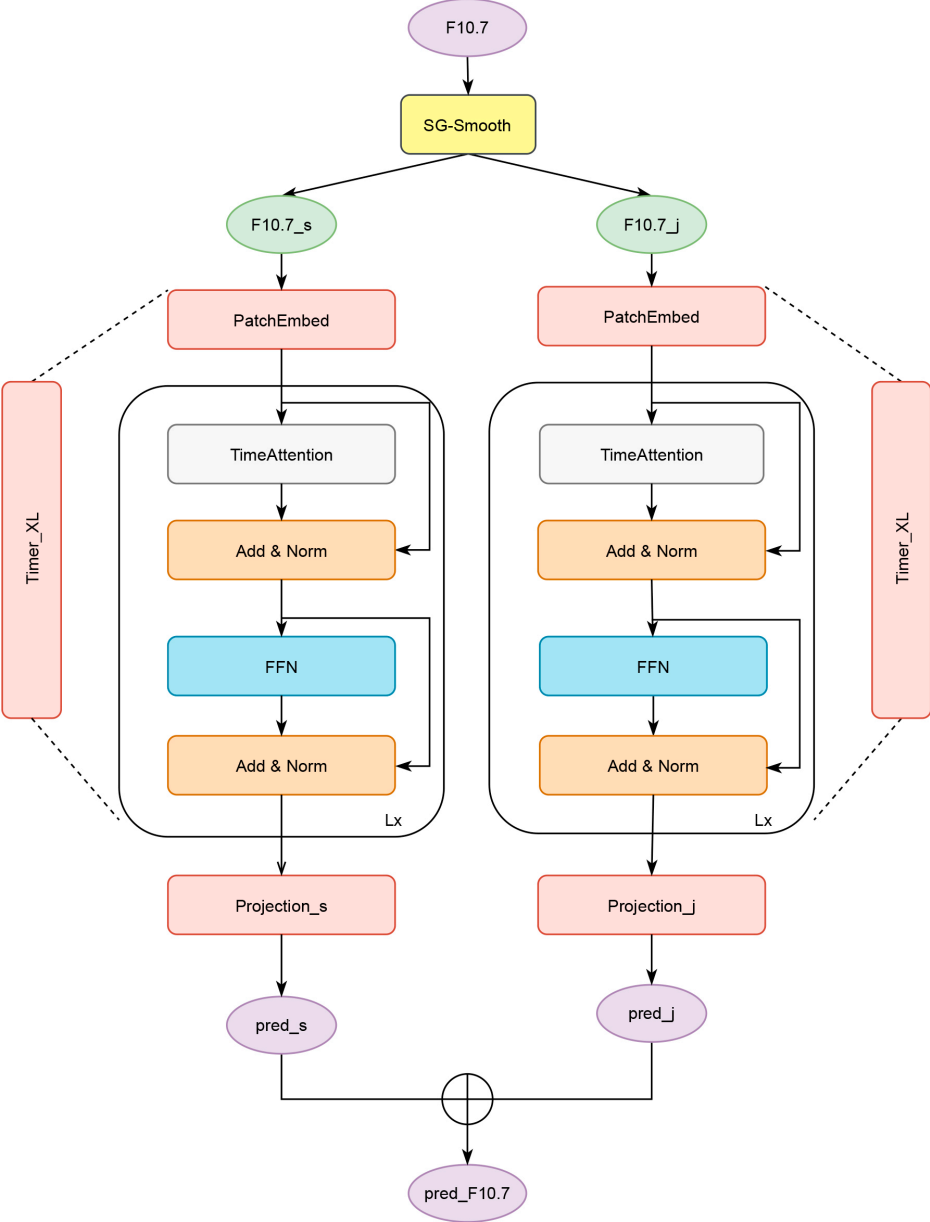
Figure 1. from Xiaolong Wang et al 2026 Astrophys. J. Suppl. 286 doi:10.3847/1538-4365/ae9096 https://dx.doi.org/10.3847/1538-4365/ae9096 © 2026. The Author(s). Published by the American Astronomical Society.
