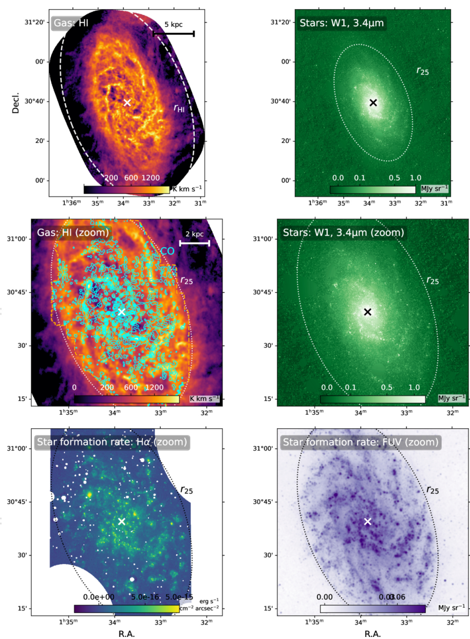
Figure 9. from Cosima Eibensteiner et al 2026 Astrophys. J. Suppl. 286 doi:10.3847/1538-4365/ae9080 https://dx.doi.org/10.3847/1538-4365/ae9080 © 2026. The Author(s). Published by the American Astronomical Society.
