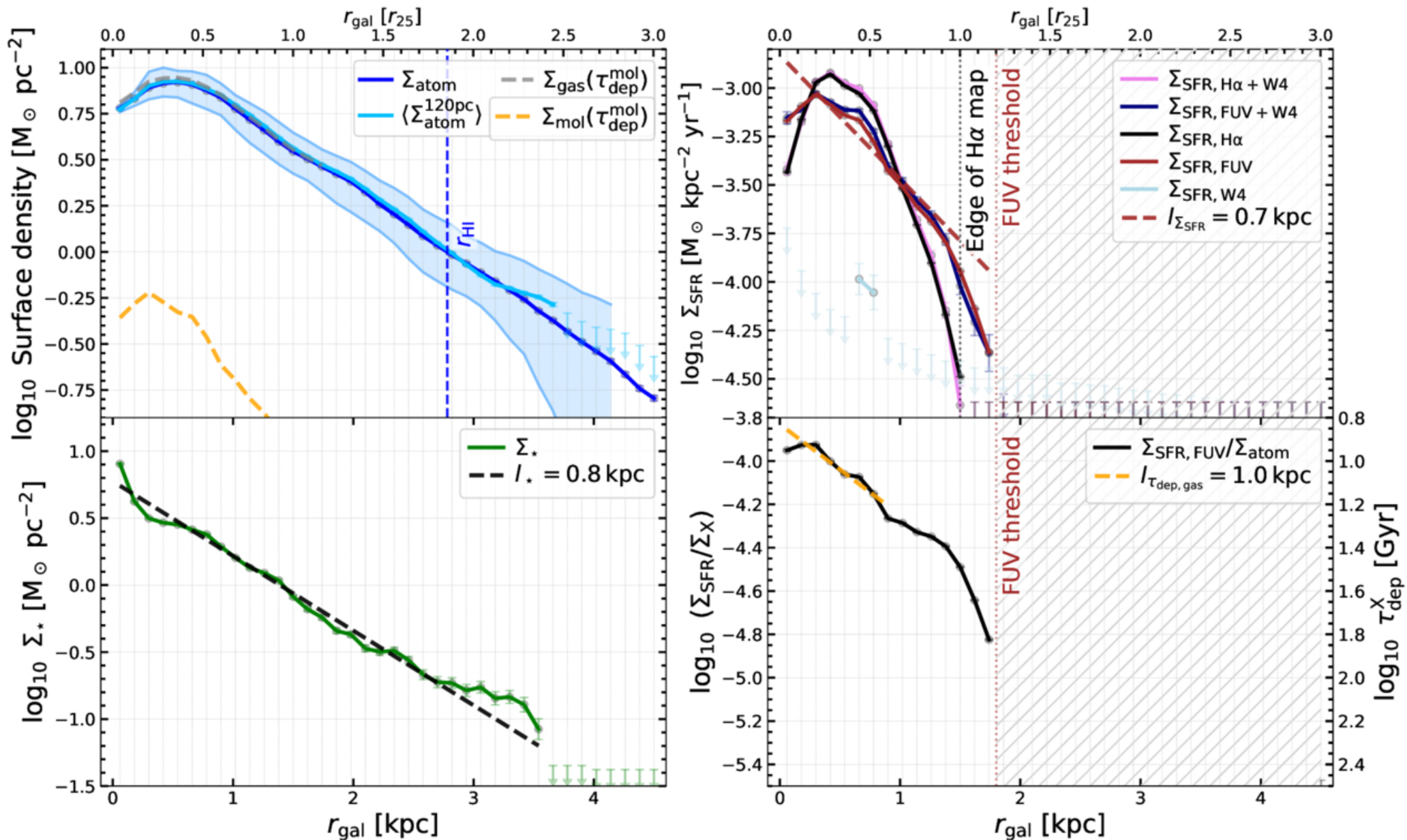
Figure 8. from Cosima Eibensteiner et al 2026 Astrophys. J. Suppl. 286 doi:10.3847/1538-4365/ae9080 https://dx.doi.org/10.3847/1538-4365/ae9080 © 2026. The Author(s). Published by the American Astronomical Society.
