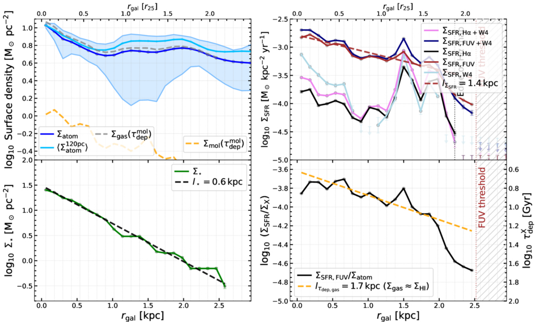
Figure 6. from Cosima Eibensteiner et al 2026 Astrophys. J. Suppl. 286 doi:10.3847/1538-4365/ae9080 https://dx.doi.org/10.3847/1538-4365/ae9080 © 2026. The Author(s). Published by the American Astronomical Society.
