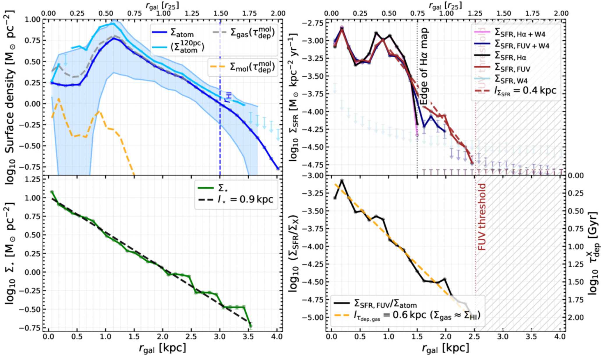
Figure 4. from Cosima Eibensteiner et al 2026 Astrophys. J. Suppl. 286 doi:10.3847/1538-4365/ae9080 https://dx.doi.org/10.3847/1538-4365/ae9080 © 2026. The Author(s). Published by the American Astronomical Society.
