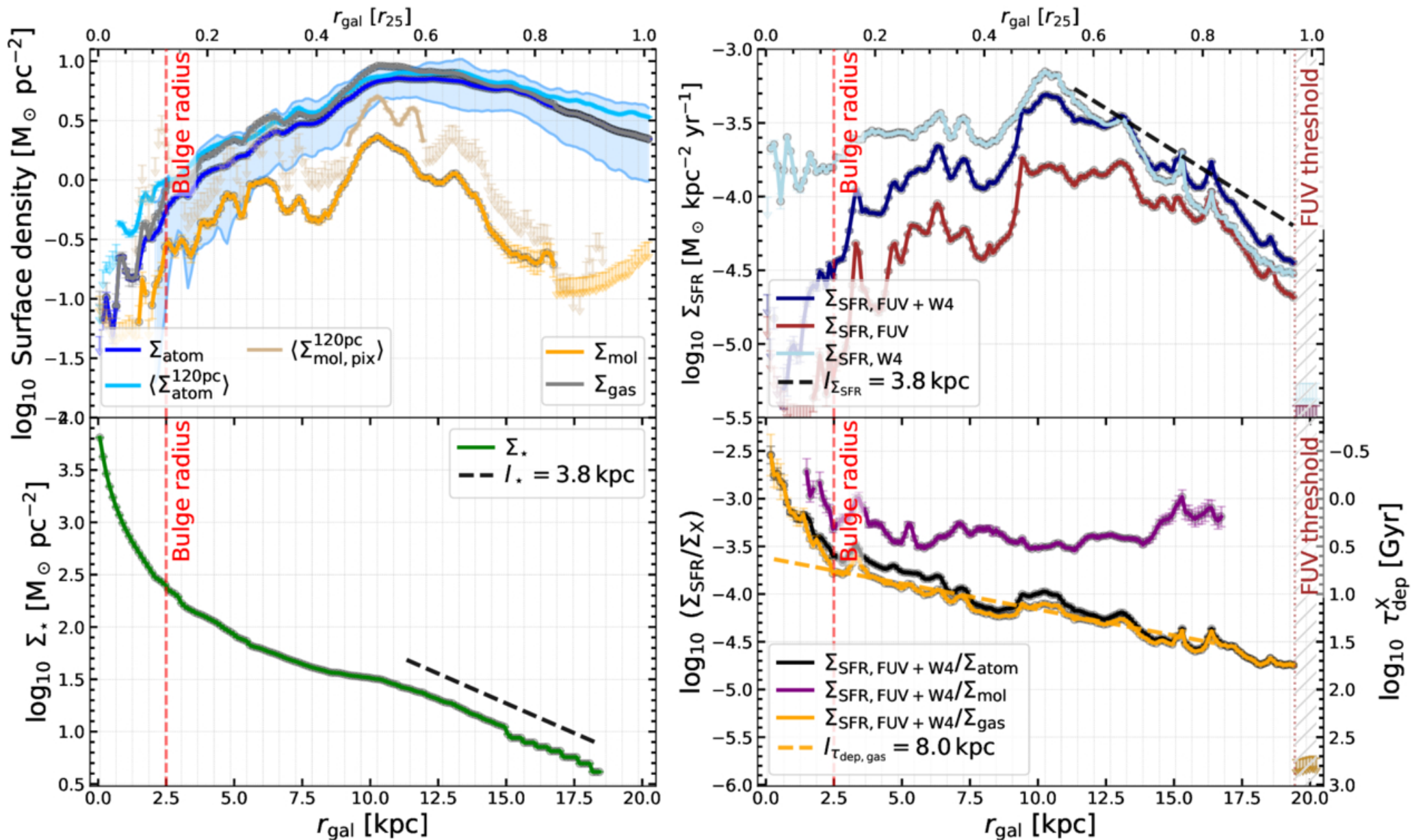
Figure 12. from Cosima Eibensteiner et al 2026 Astrophys. J. Suppl. 286 doi:10.3847/1538-4365/ae9080 https://dx.doi.org/10.3847/1538-4365/ae9080 © 2026. The Author(s). Published by the American Astronomical Society.
