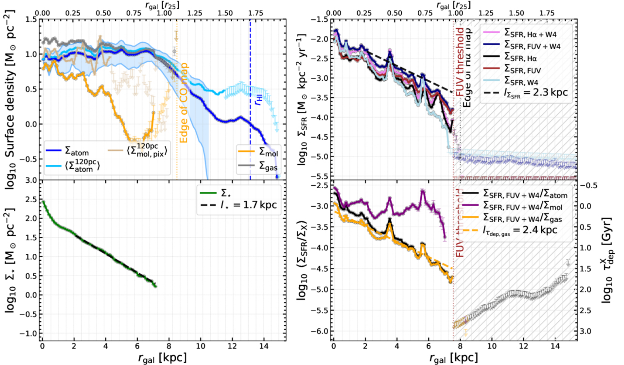
Figure 10. from Cosima Eibensteiner et al 2026 Astrophys. J. Suppl. 286 doi:10.3847/1538-4365/ae9080 https://dx.doi.org/10.3847/1538-4365/ae9080 © 2026. The Author(s). Published by the American Astronomical Society.
