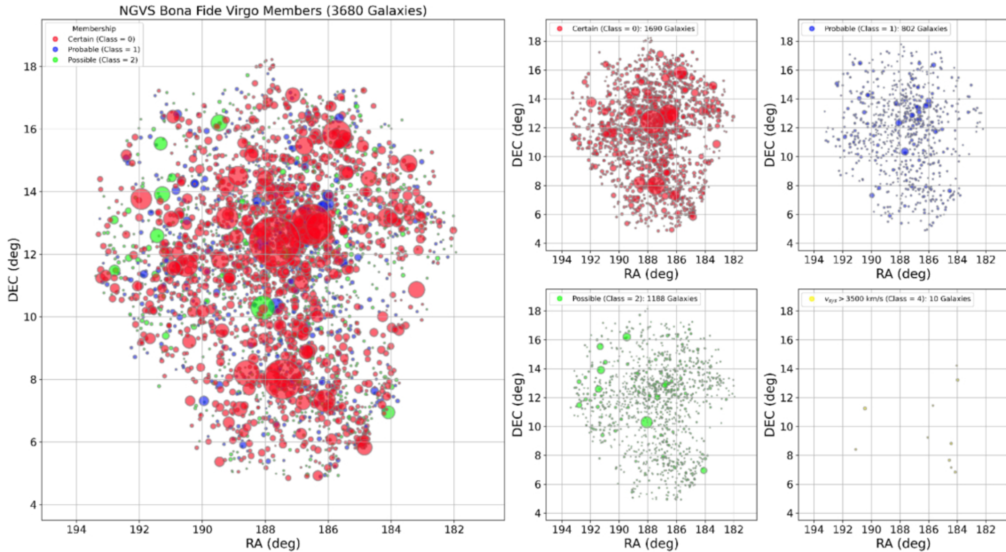
Figure 9. from Laura Ferrarese et al 2026 Astrophys. J. Suppl. 286 doi:10.3847/1538-4365/ae8fc7 https://dx.doi.org/10.3847/1538-4365/ae8fc7 © 2026. The Author(s). Published by the American Astronomical Society.
