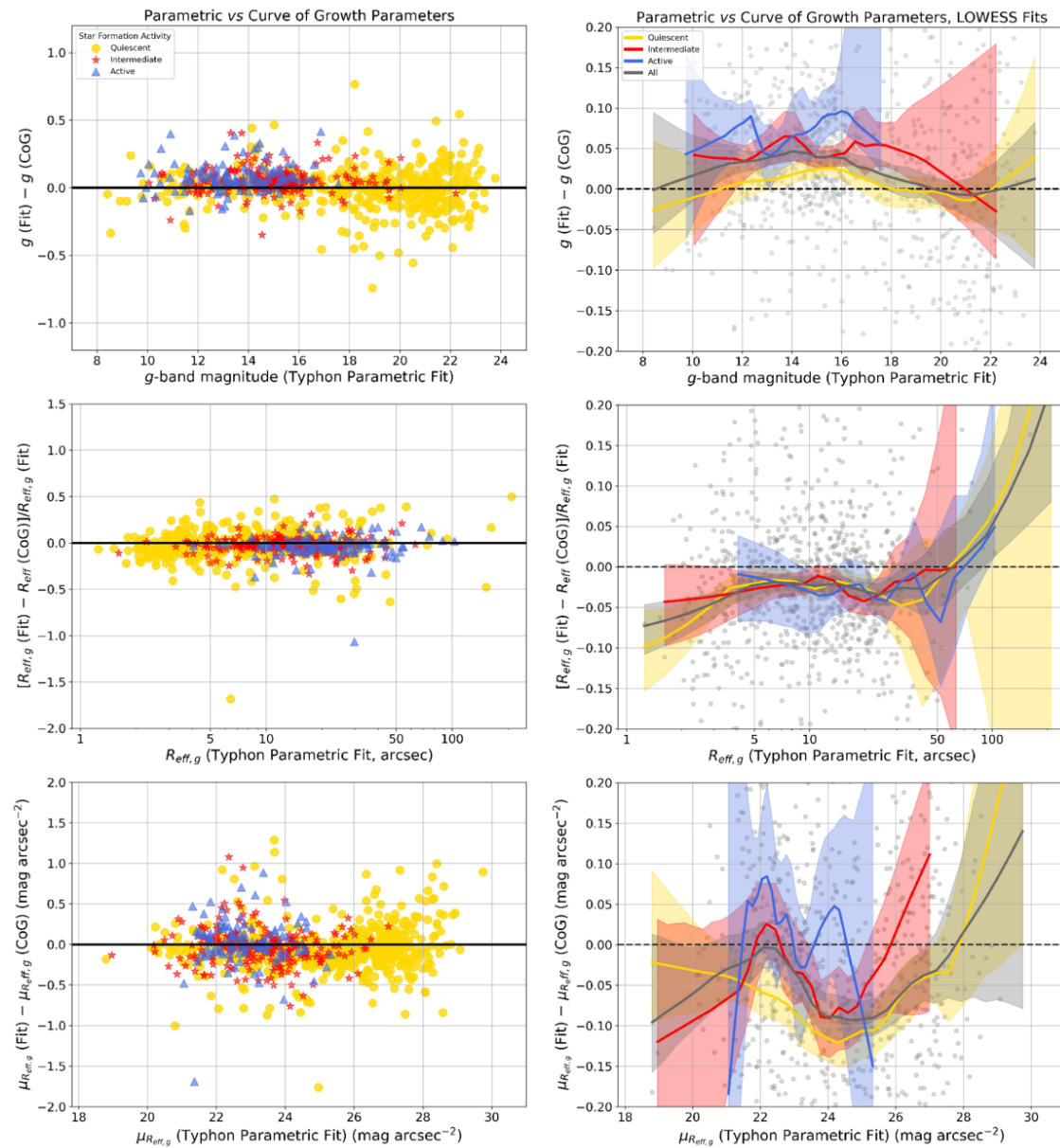
Figure 20. from Laura Ferrarese et al 2026 Astrophys. J. Suppl. 286 doi:10.3847/1538-4365/ae8fc7 https://dx.doi.org/10.3847/1538-4365/ae8fc7 © 2026. The Author(s). Published by the American Astronomical Society.
