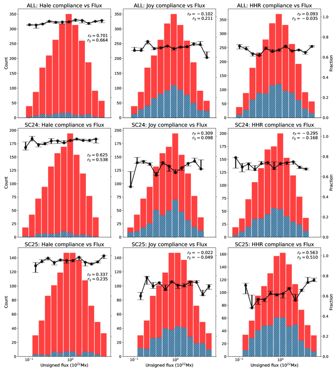
Figure 6. from Jinhui Pan et al 2026 Astrophys. J. Suppl. 285 doi:10.3847/1538-4365/ae88ee https://dx.doi.org/10.3847/1538-4365/ae88ee © 2026. The Author(s). Published by the American Astronomical Society.
