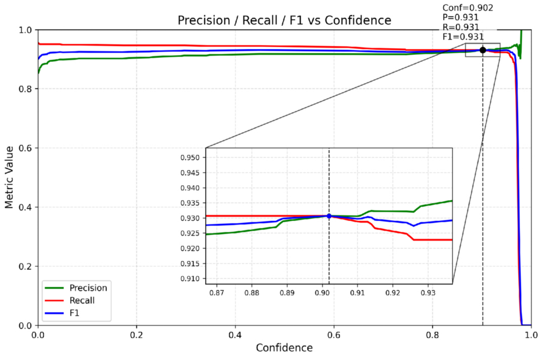
Figure 4. from Yuechang Liu et al 2026 Astrophys. J. Suppl. 285 doi:10.3847/1538-4365/ae8849 https://dx.doi.org/10.3847/1538-4365/ae8849 © 2026. The Author(s). Published by the American Astronomical Society.
