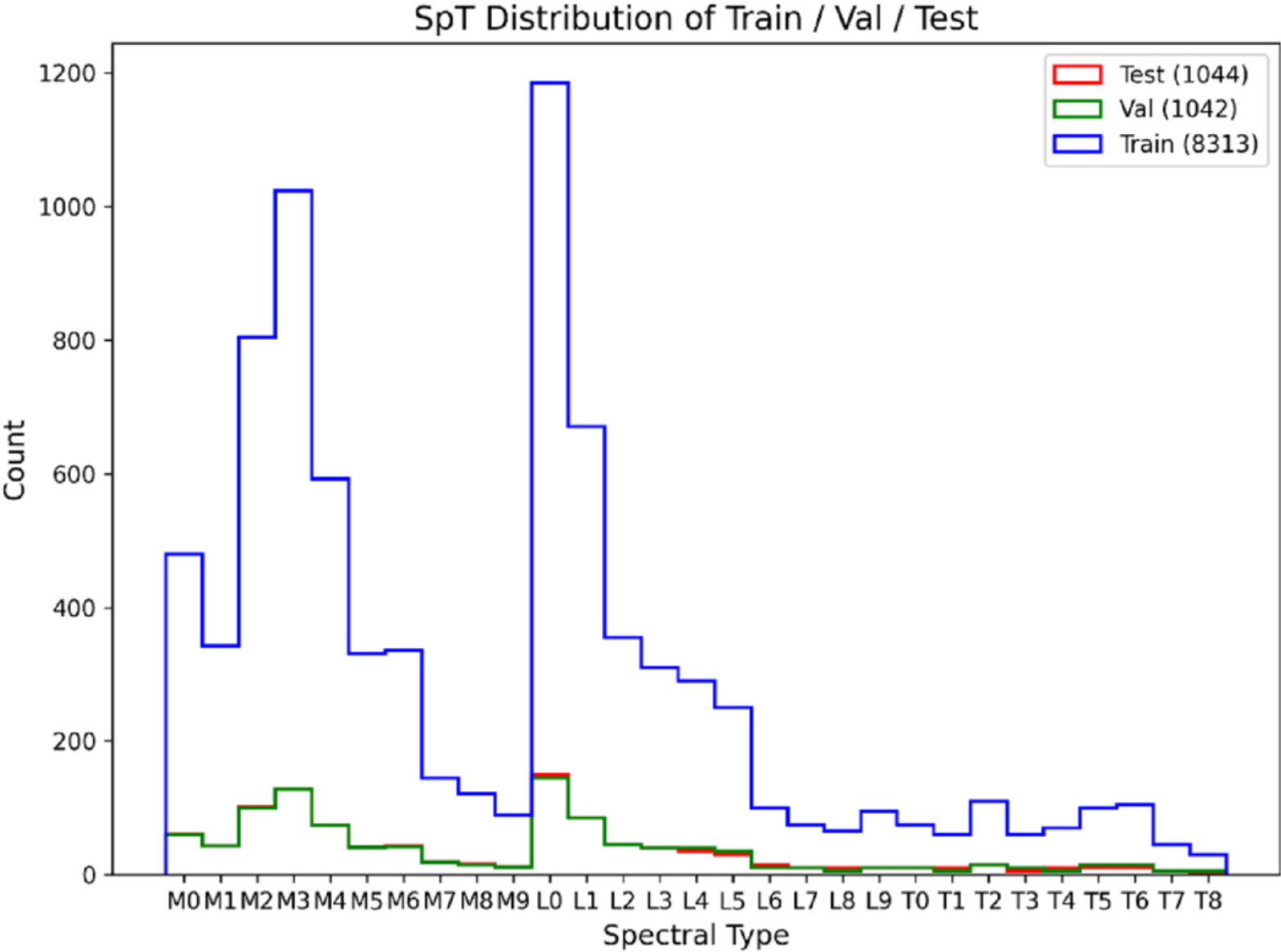
Figure 2. from Yuechang Liu et al 2026 Astrophys. J. Suppl. 285 doi:10.3847/1538-4365/ae8849 https://dx.doi.org/10.3847/1538-4365/ae8849 © 2026. The Author(s). Published by the American Astronomical Society.
