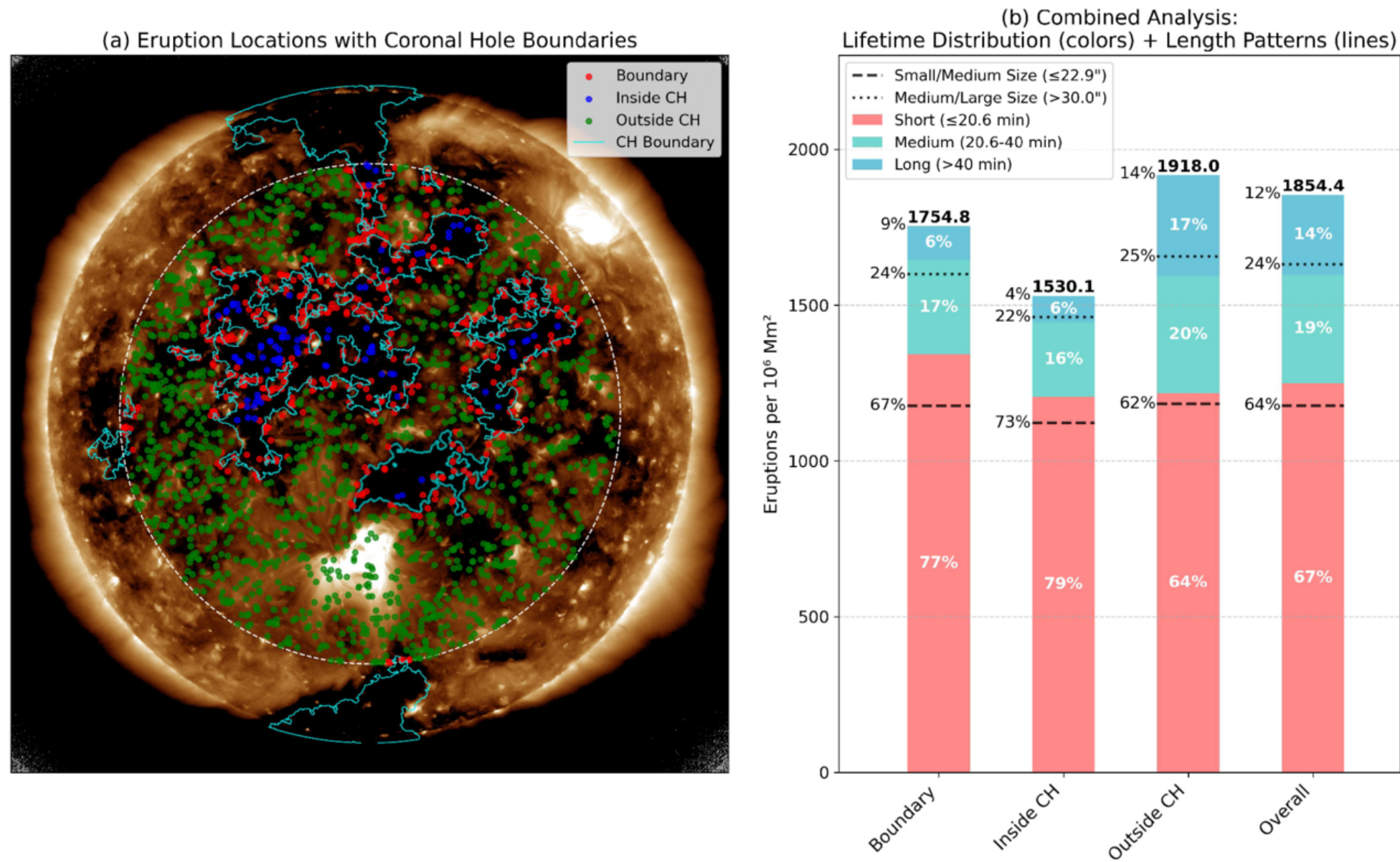
Figure 9. from Artin Khaleghi et al 2026 Astrophys. J. Suppl. 285 doi:10.3847/1538-4365/ae8844 https://dx.doi.org/10.3847/1538-4365/ae8844 © 2026. The Author(s). Published by the American Astronomical Society.
