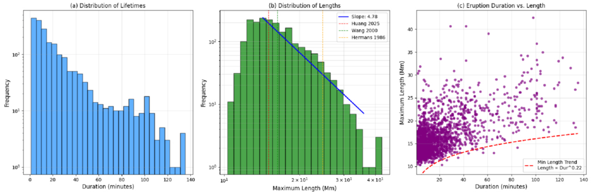
Figure 8. from Artin Khaleghi et al 2026 Astrophys. J. Suppl. 285 doi:10.3847/1538-4365/ae8844 https://dx.doi.org/10.3847/1538-4365/ae8844 © 2026. The Author(s). Published by the American Astronomical Society.
