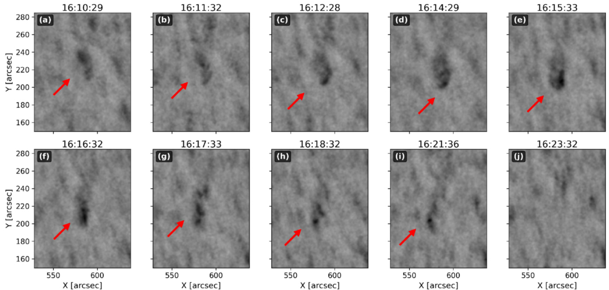
Figure 6. from Artin Khaleghi et al 2026 Astrophys. J. Suppl. 285 doi:10.3847/1538-4365/ae8844 https://dx.doi.org/10.3847/1538-4365/ae8844 © 2026. The Author(s). Published by the American Astronomical Society.
