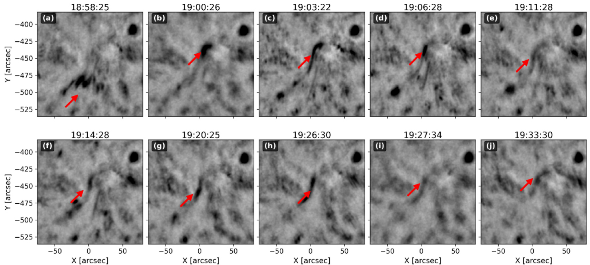
Figure 5. from Artin Khaleghi et al 2026 Astrophys. J. Suppl. 285 doi:10.3847/1538-4365/ae8844 https://dx.doi.org/10.3847/1538-4365/ae8844 © 2026. The Author(s). Published by the American Astronomical Society.
