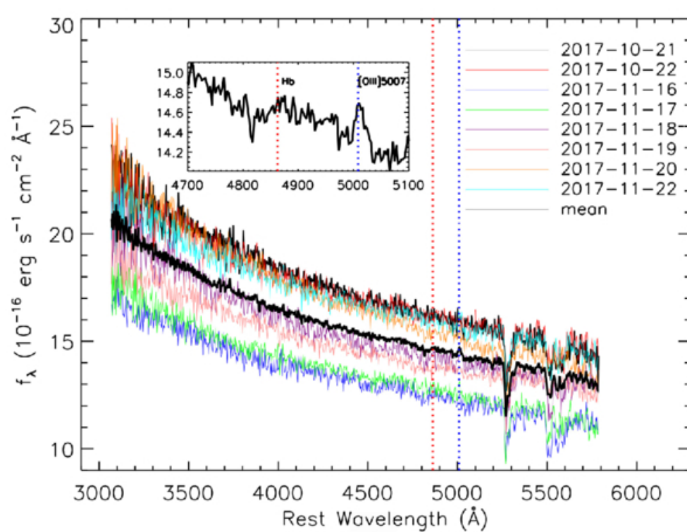
Figure 5. from Alok C. Gupta et al 2026 Astrophys. J. Suppl. 286 doi:10.3847/1538-4365/ae8795 https://dx.doi.org/10.3847/1538-4365/ae8795 © 2026. The Author(s). Published by the American Astronomical Society.
