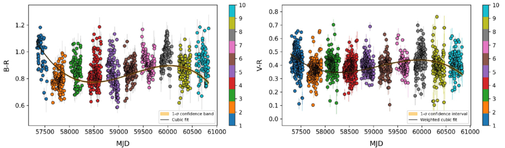
Figure 3. from Alok C. Gupta et al 2026 Astrophys. J. Suppl. 286 doi:10.3847/1538-4365/ae8795 https://dx.doi.org/10.3847/1538-4365/ae8795 © 2026. The Author(s). Published by the American Astronomical Society.
