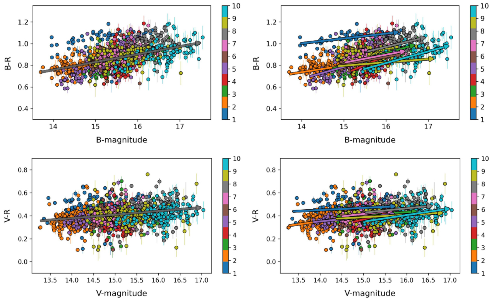
Figure 2. from Alok C. Gupta et al 2026 Astrophys. J. Suppl. 286 doi:10.3847/1538-4365/ae8795 https://dx.doi.org/10.3847/1538-4365/ae8795 © 2026. The Author(s). Published by the American Astronomical Society.
