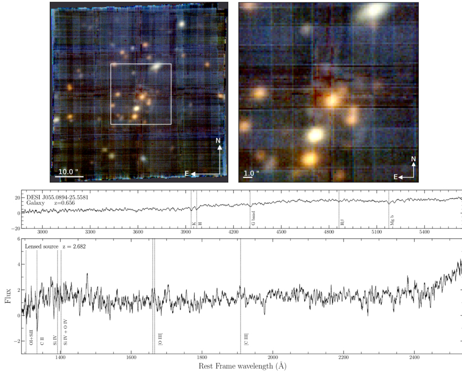
Figure 8. from Emerald Lin et al 2026 Astrophys. J. Suppl. 286 doi:10.3847/1538-4365/ae844d https://dx.doi.org/10.3847/1538-4365/ae844d © 2026. The Author(s). Published by the American Astronomical Society.
