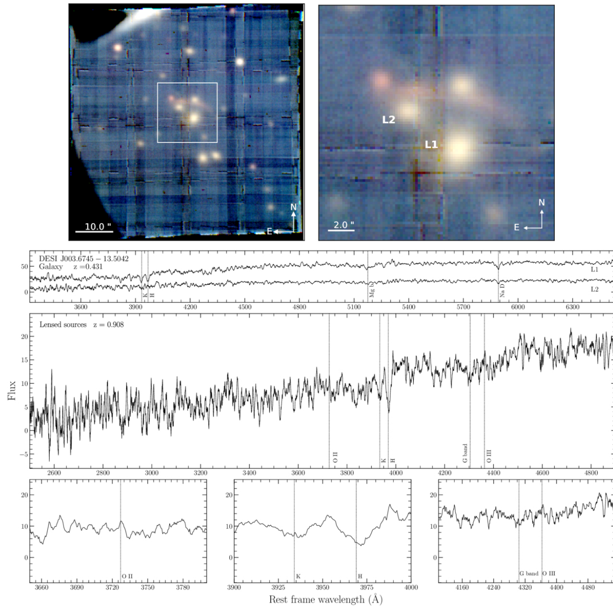
Figure 3. from Emerald Lin et al 2026 Astrophys. J. Suppl. 286 doi:10.3847/1538-4365/ae844d https://dx.doi.org/10.3847/1538-4365/ae844d © 2026. The Author(s). Published by the American Astronomical Society.
