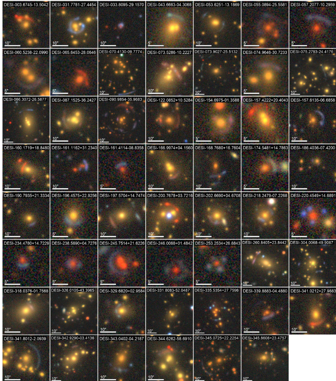
Figure 2. from Emerald Lin et al 2026 Astrophys. J. Suppl. 286 doi:10.3847/1538-4365/ae844d https://dx.doi.org/10.3847/1538-4365/ae844d © 2026. The Author(s). Published by the American Astronomical Society.
