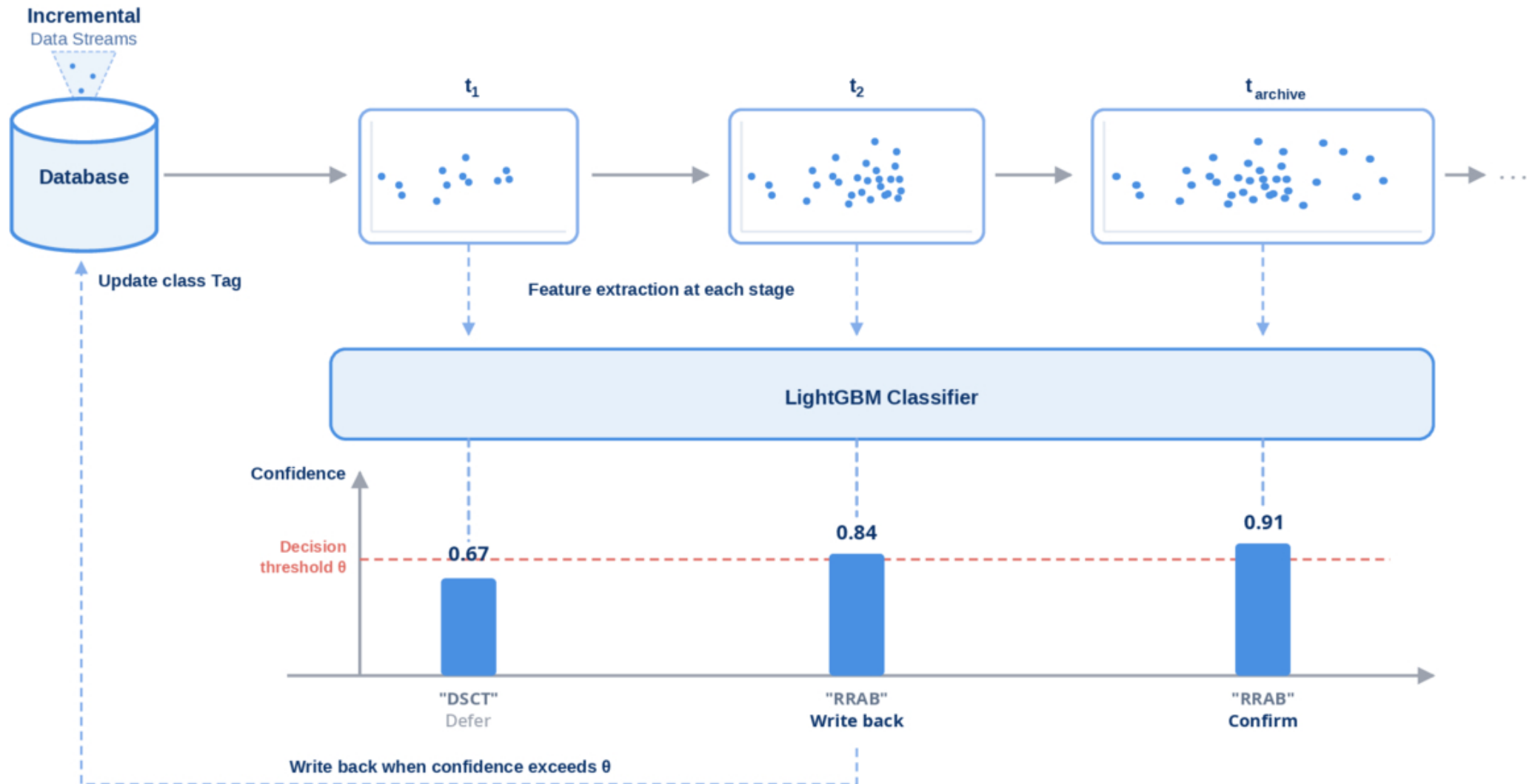
Figure 7. from Xinghang Yu et al 2026 Astrophys. J. Suppl. 285 doi:10.3847/1538-4365/ae8300 https://dx.doi.org/10.3847/1538-4365/ae8300 © 2026. The Author(s). Published by the American Astronomical Society.
