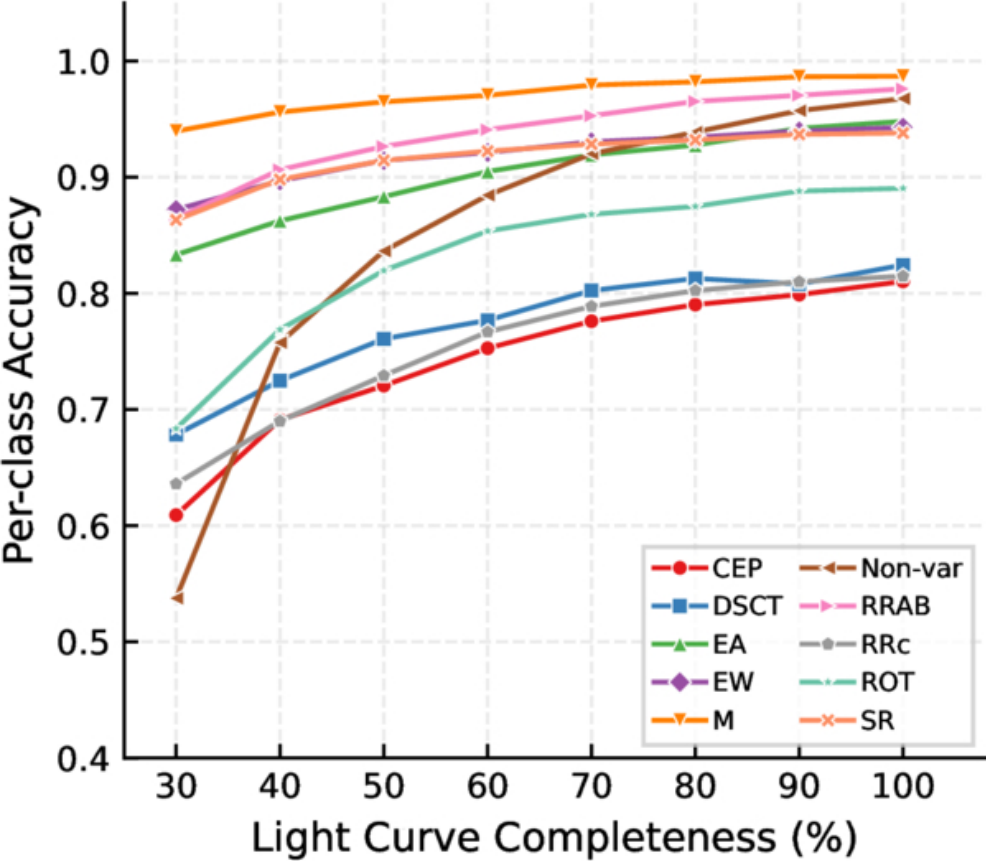
Figure 6. from Xinghang Yu et al 2026 Astrophys. J. Suppl. 285 doi:10.3847/1538-4365/ae8300 https://dx.doi.org/10.3847/1538-4365/ae8300 © 2026. The Author(s). Published by the American Astronomical Society.
