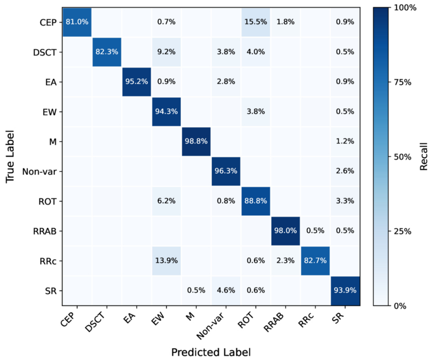
Figure 4. from Xinghang Yu et al 2026 Astrophys. J. Suppl. 285 doi:10.3847/1538-4365/ae8300 https://dx.doi.org/10.3847/1538-4365/ae8300 © 2026. The Author(s). Published by the American Astronomical Society.
