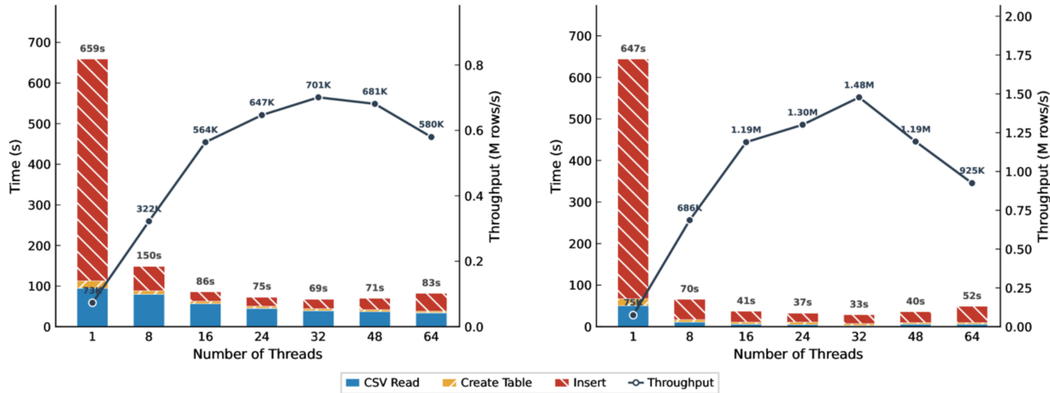
Figure 3. from Xinghang Yu et al 2026 Astrophys. J. Suppl. 285 doi:10.3847/1538-4365/ae8300 https://dx.doi.org/10.3847/1538-4365/ae8300 © 2026. The Author(s). Published by the American Astronomical Society.
