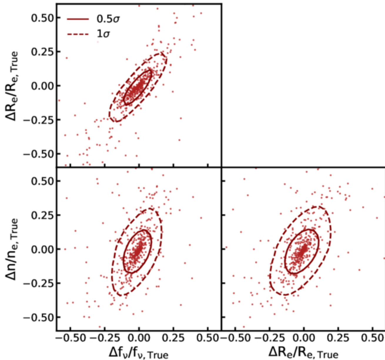
Figure 5. from Yunchong Zhang et al 2026 Astrophys. J. Suppl. 285 doi:10.3847/1538-4365/ae82f7 https://dx.doi.org/10.3847/1538-4365/ae82f7 © 2026. The Author(s). Published by the American Astronomical Society.
