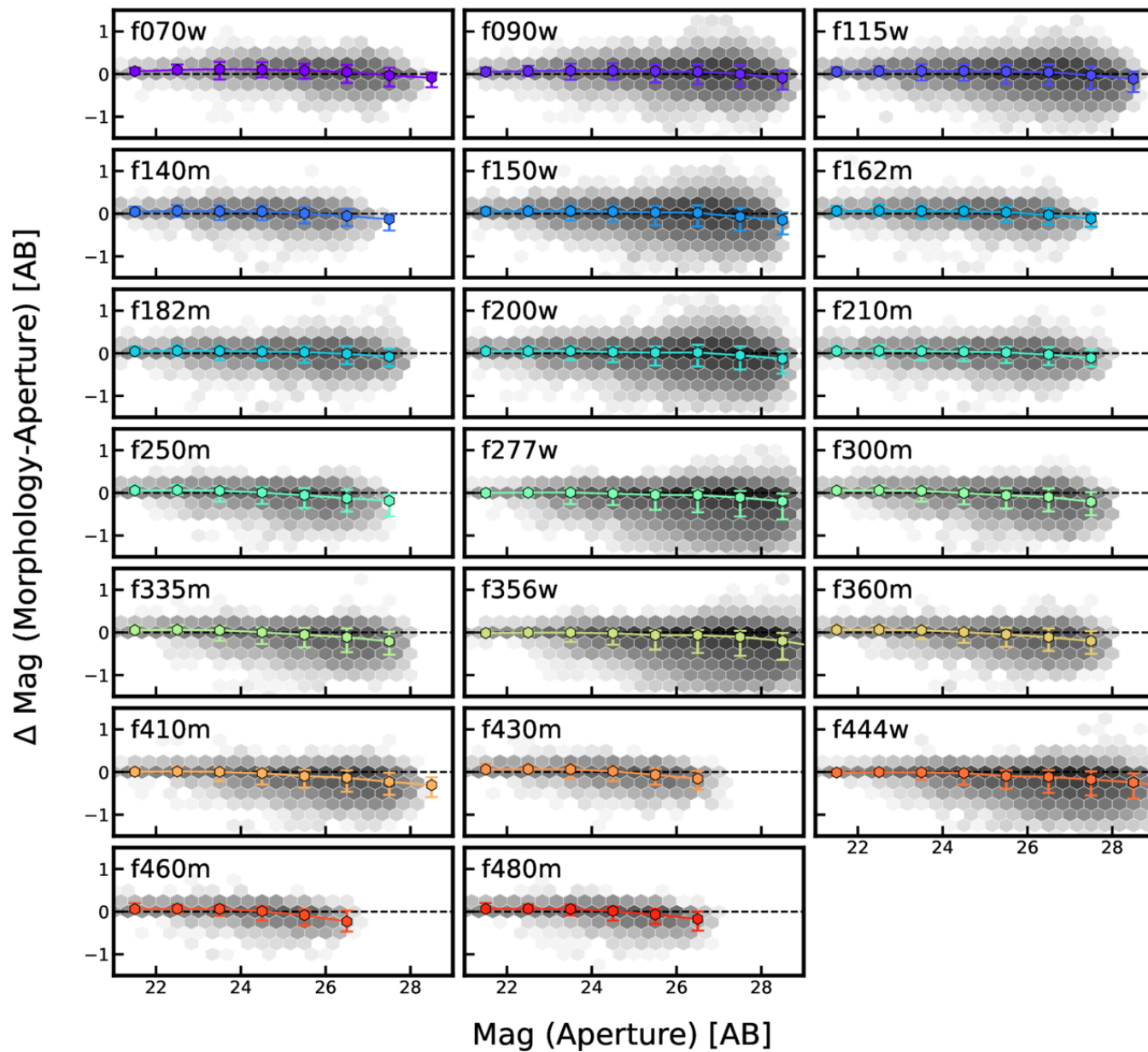
Figure 3. from Yunchong Zhang et al 2026 Astrophys. J. Suppl. 285 doi:10.3847/1538-4365/ae82f7 https://dx.doi.org/10.3847/1538-4365/ae82f7 © 2026. The Author(s). Published by the American Astronomical Society.
