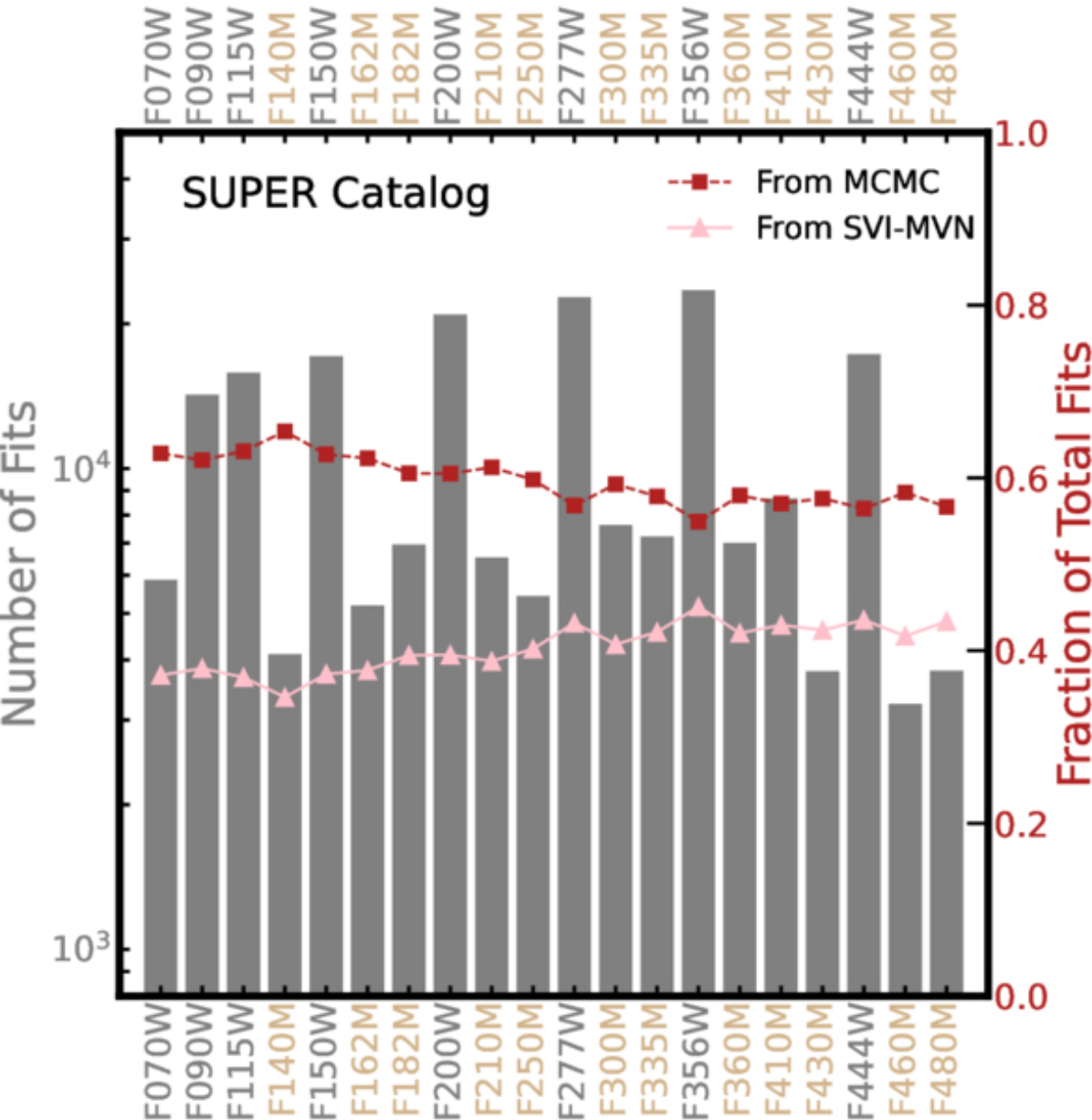
Figure 2. from Yunchong Zhang et al 2026 Astrophys. J. Suppl. 285 doi:10.3847/1538-4365/ae82f7 https://dx.doi.org/10.3847/1538-4365/ae82f7 © 2026. The Author(s). Published by the American Astronomical Society.
