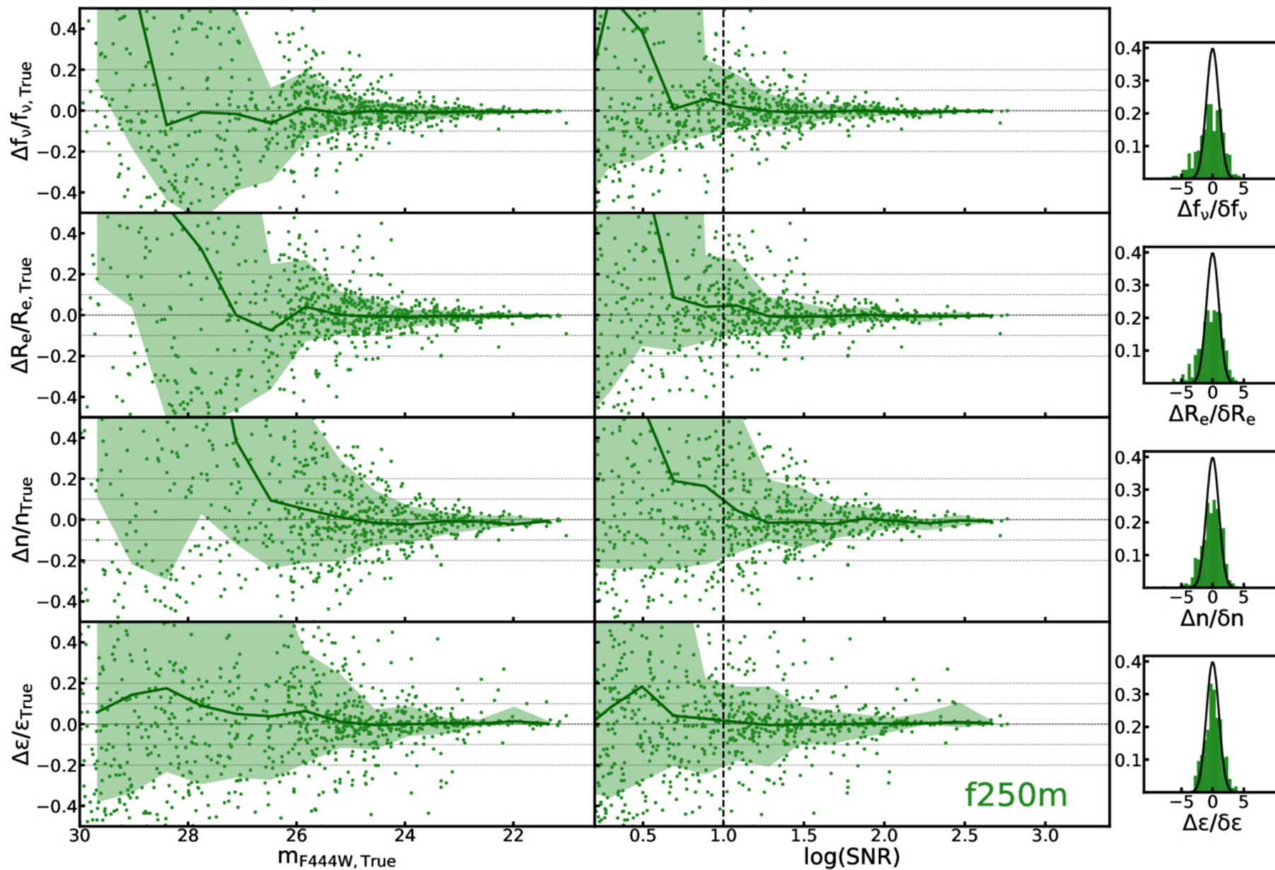
Figure 12. from Yunchong Zhang et al 2026 Astrophys. J. Suppl. 285 doi:10.3847/1538-4365/ae82f7 https://dx.doi.org/10.3847/1538-4365/ae82f7 © 2026. The Author(s). Published by the American Astronomical Society.
