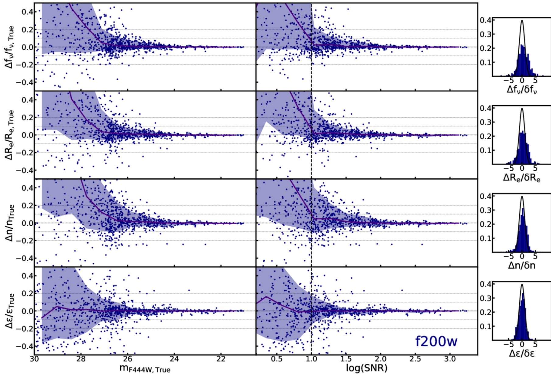
Figure 11. from Yunchong Zhang et al 2026 Astrophys. J. Suppl. 285 doi:10.3847/1538-4365/ae82f7 https://dx.doi.org/10.3847/1538-4365/ae82f7 © 2026. The Author(s). Published by the American Astronomical Society.
