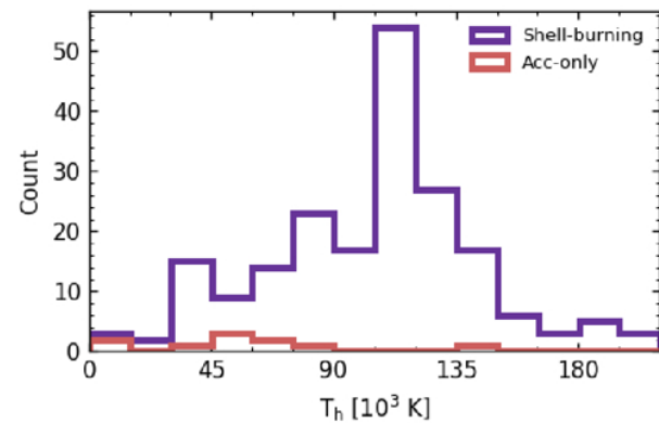
Figure 5. from Jaroslav Merc et al 2026 Astrophys. J. Suppl. 285 doi:10.3847/1538-4365/ae82ee https://dx.doi.org/10.3847/1538-4365/ae82ee © 2026. The Author(s). Published by the American Astronomical Society.
