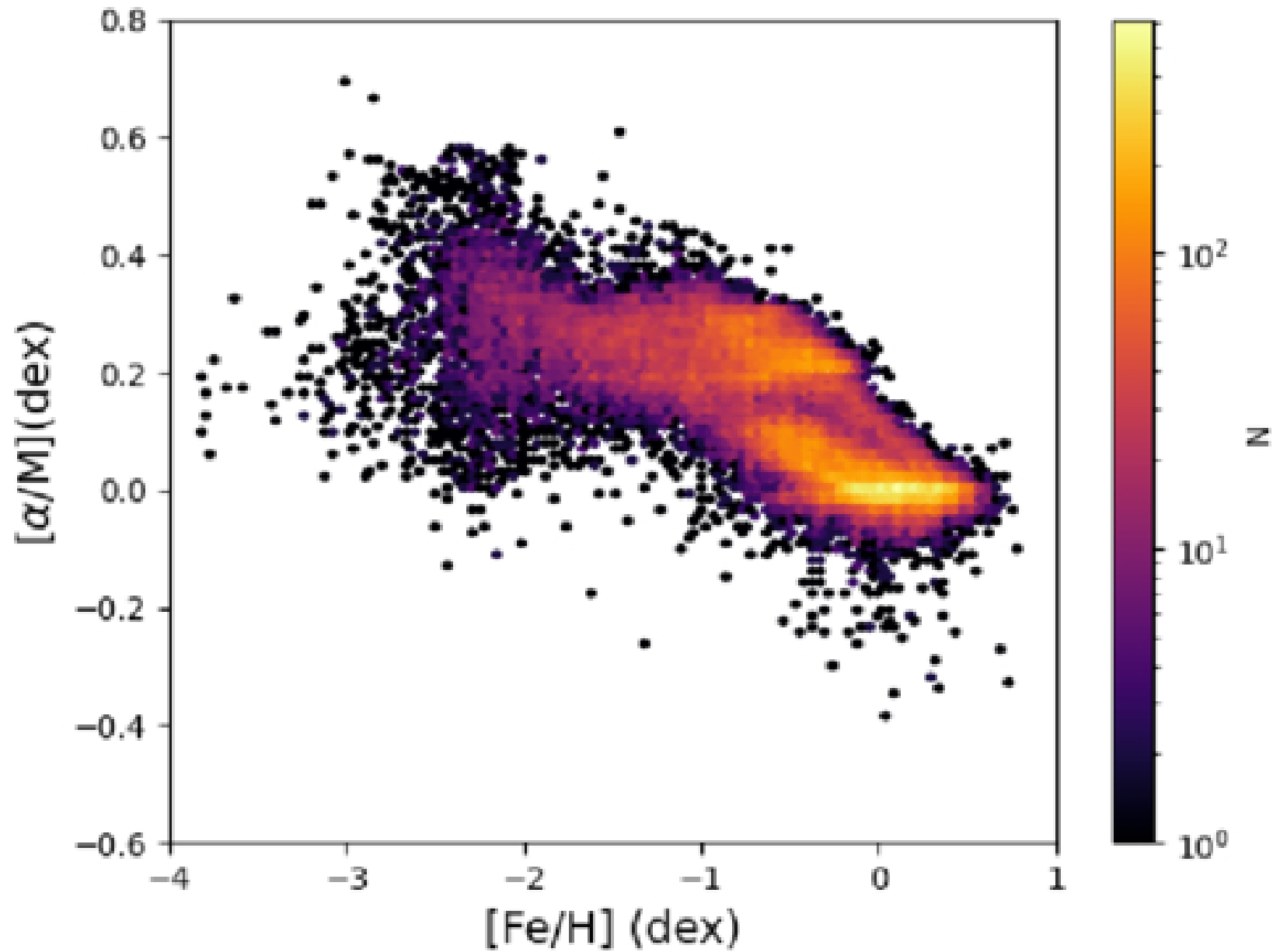
Figure 8. from Bing Du et al 2026 Astrophys. J. Suppl. 285 doi:10.3847/1538-4365/ae81b7 https://dx.doi.org/10.3847/1538-4365/ae81b7 © 2026. The Author(s). Published by the American Astronomical Society.
