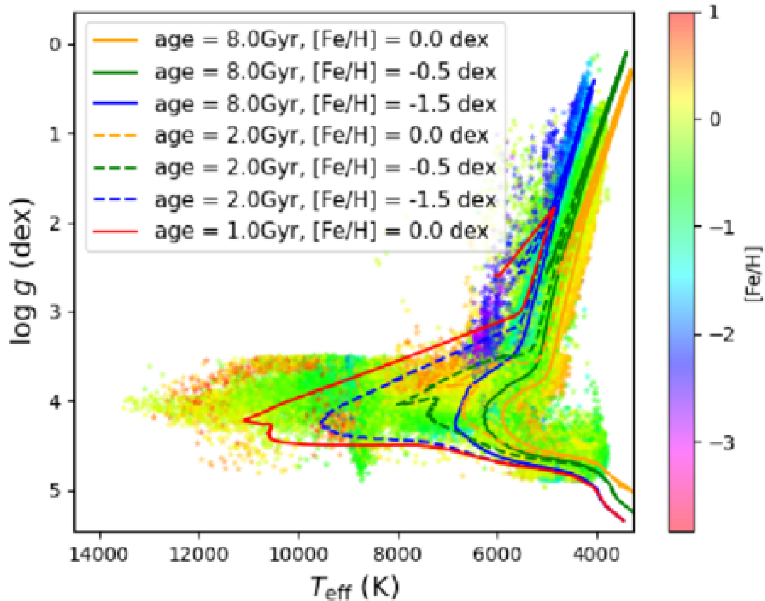
Figure 7. from Bing Du et al 2026 Astrophys. J. Suppl. 285 doi:10.3847/1538-4365/ae81b7 https://dx.doi.org/10.3847/1538-4365/ae81b7 © 2026. The Author(s). Published by the American Astronomical Society.
