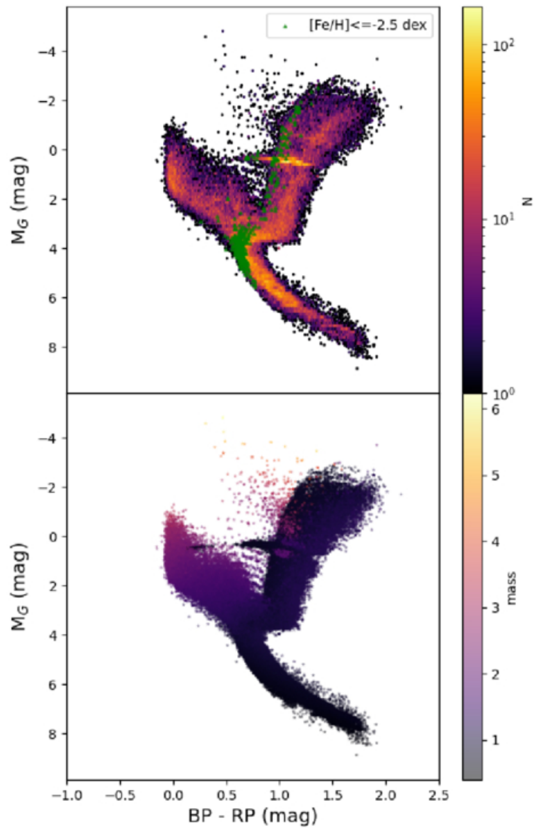
Figure 6. from Bing Du et al 2026 Astrophys. J. Suppl. 285 doi:10.3847/1538-4365/ae81b7 https://dx.doi.org/10.3847/1538-4365/ae81b7 © 2026. The Author(s). Published by the American Astronomical Society.
