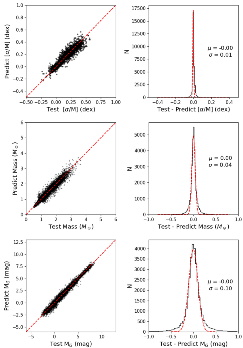
Figure 5. from Bing Du et al 2026 Astrophys. J. Suppl. 285 doi:10.3847/1538-4365/ae81b7 https://dx.doi.org/10.3847/1538-4365/ae81b7 © 2026. The Author(s). Published by the American Astronomical Society.
