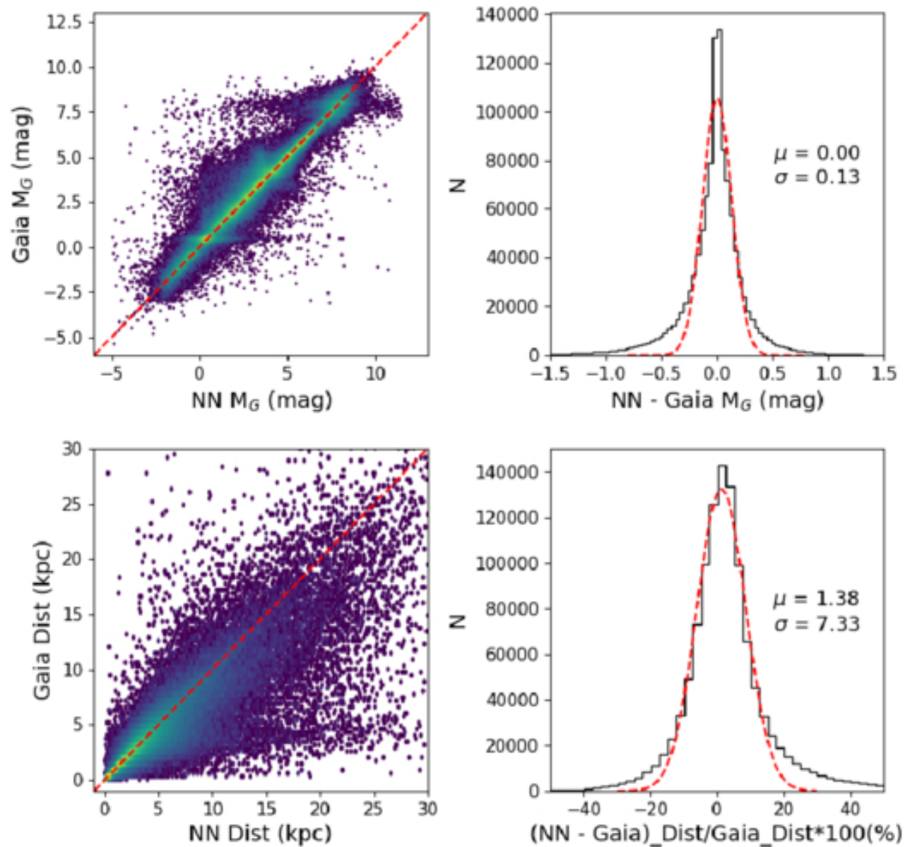
Figure 19. from Bing Du et al 2026 Astrophys. J. Suppl. 285 doi:10.3847/1538-4365/ae81b7 https://dx.doi.org/10.3847/1538-4365/ae81b7 © 2026. The Author(s). Published by the American Astronomical Society.
