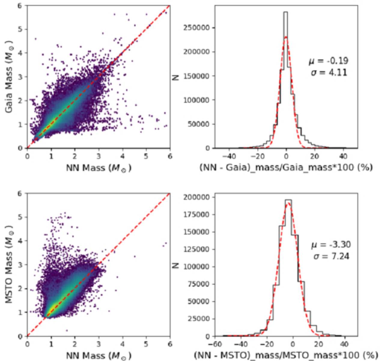
Figure 18. from Bing Du et al 2026 Astrophys. J. Suppl. 285 doi:10.3847/1538-4365/ae81b7 https://dx.doi.org/10.3847/1538-4365/ae81b7 © 2026. The Author(s). Published by the American Astronomical Society.
