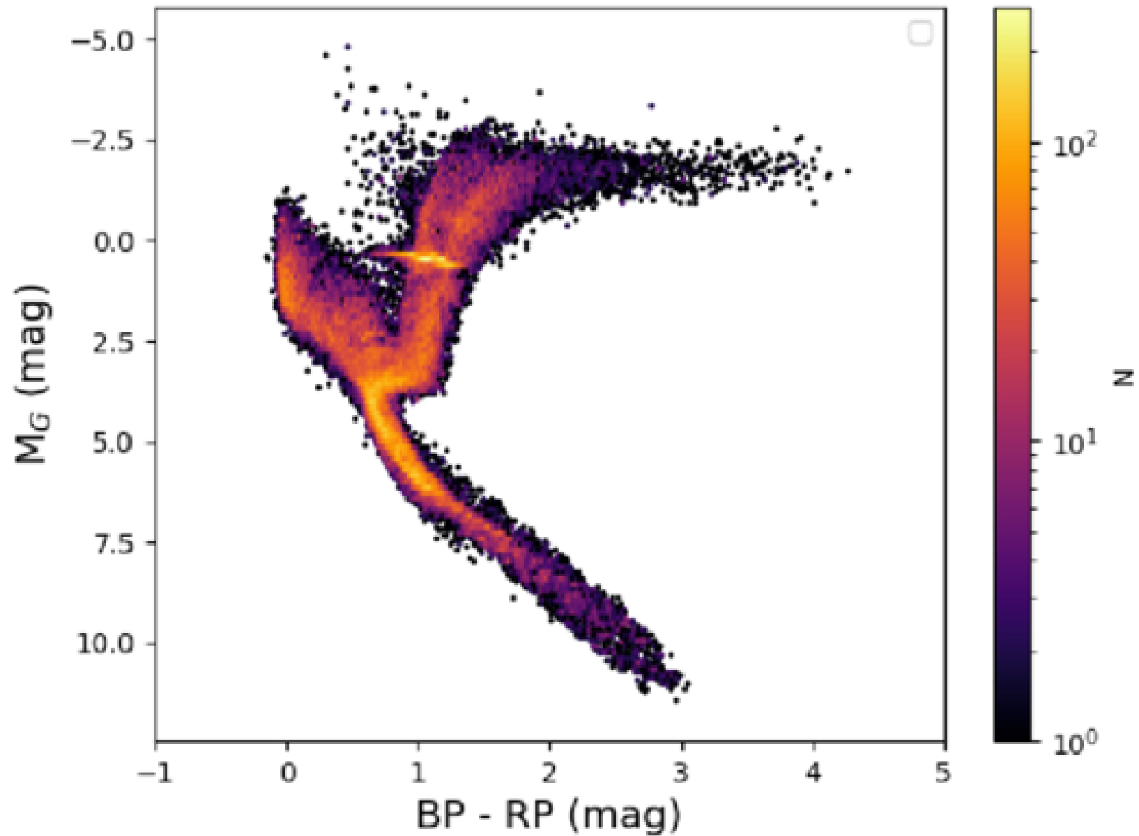
Figure 11. from Bing Du et al 2026 Astrophys. J. Suppl. 285 doi:10.3847/1538-4365/ae81b7 https://dx.doi.org/10.3847/1538-4365/ae81b7 © 2026. The Author(s). Published by the American Astronomical Society.
