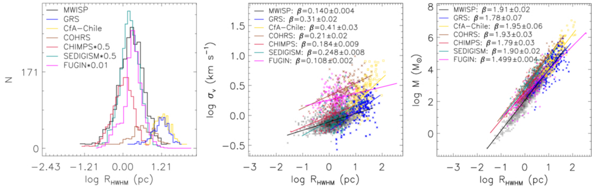
Figure 7. from Xin Zhou et al 2026 Astrophys. J. Suppl. 285 doi:10.3847/1538-4365/ae8155 https://dx.doi.org/10.3847/1538-4365/ae8155 © 2026. The Author(s). Published by the American Astronomical Society.
