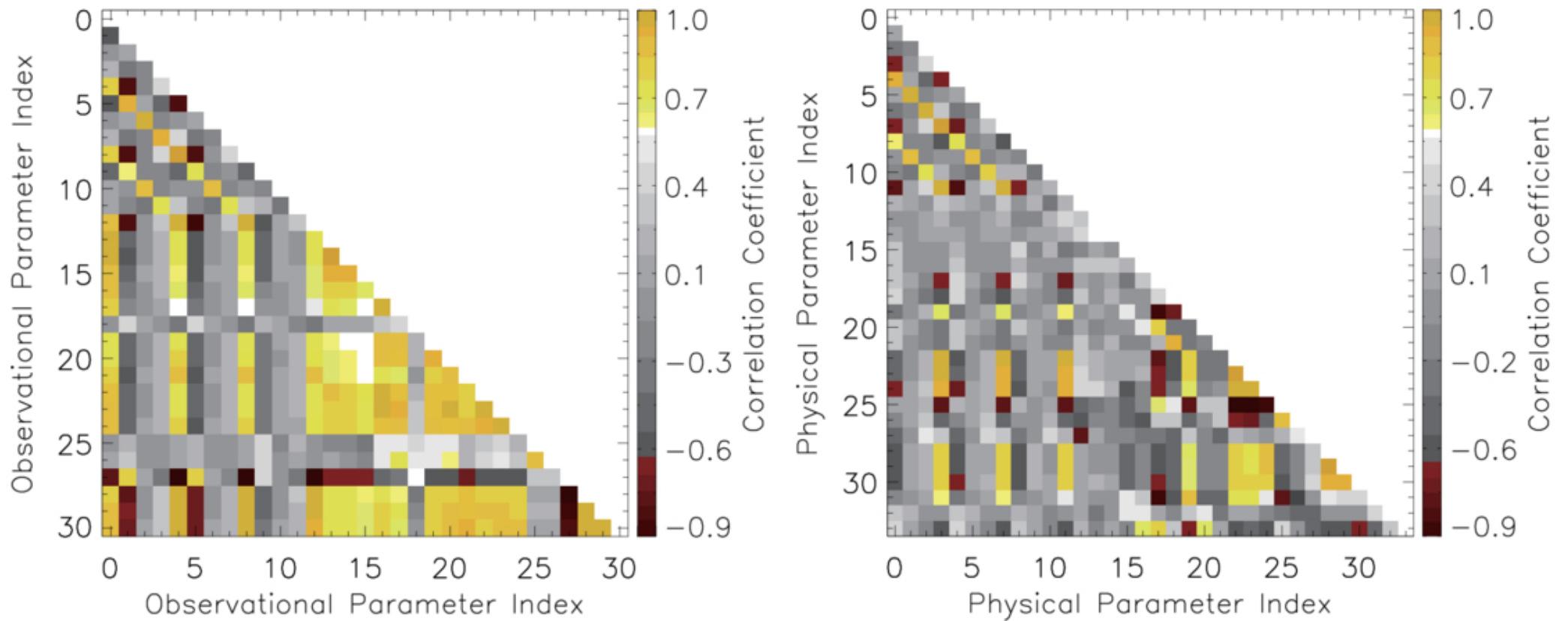
Figure 6. from Xin Zhou et al 2026 Astrophys. J. Suppl. 285 doi:10.3847/1538-4365/ae8155 https://dx.doi.org/10.3847/1538-4365/ae8155 © 2026. The Author(s). Published by the American Astronomical Society.
