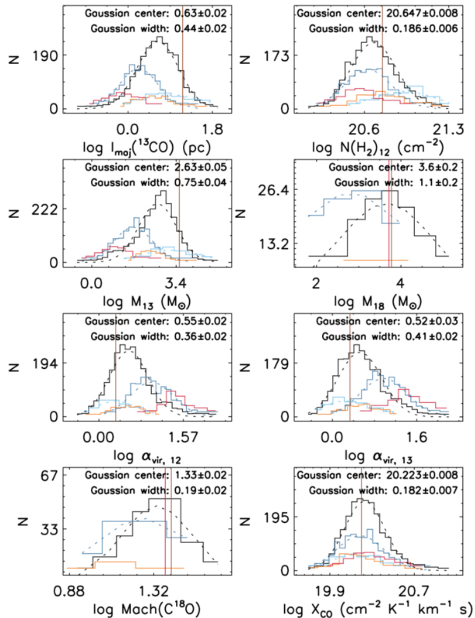
Figure 4. from Xin Zhou et al 2026 Astrophys. J. Suppl. 285 doi:10.3847/1538-4365/ae8155 https://dx.doi.org/10.3847/1538-4365/ae8155 © 2026. The Author(s). Published by the American Astronomical Society.
